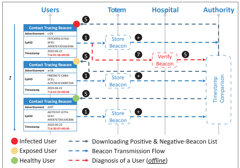
FIGURE 3. The IoTrace protocol data flow diagram. An exposed user becomes yellow if he/she is close to an infected user based on the BLE beacon's timestamp.
